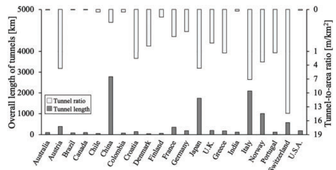
Figure 1. Motorway and railway tunnel length and tunnel-to-area ratio for some countries worldwide (modified from De Feudis et al., 14 )
